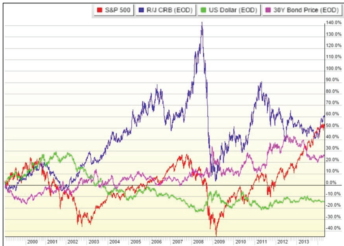
2: PerfChart: SPX, CRB, DI, CRB; 01 January 1999–01 April 2014 Source: Own source
