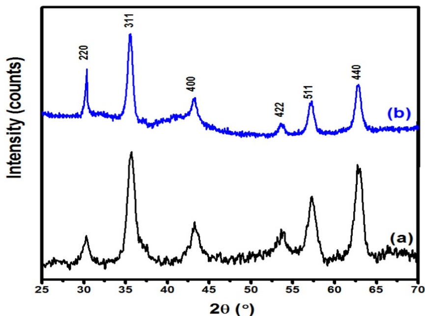
Figure 2. XRD profile of Fe 3 O 4 (a) MH and (b) MNP's at room temperature
