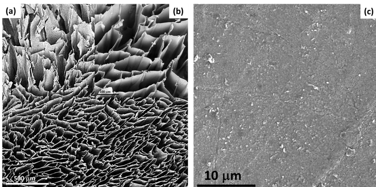
Figure 3 SEM image (a) Hydrogel, (b) high resolution image of the hydrogel (internal struc-morphology) showing the network structure and (c) Surface morphology of biomaterialized (Fe 3 O 4 ) hydrogel
