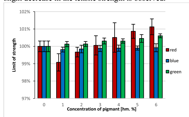
Fig 8. Proportional graph Limit of strength
