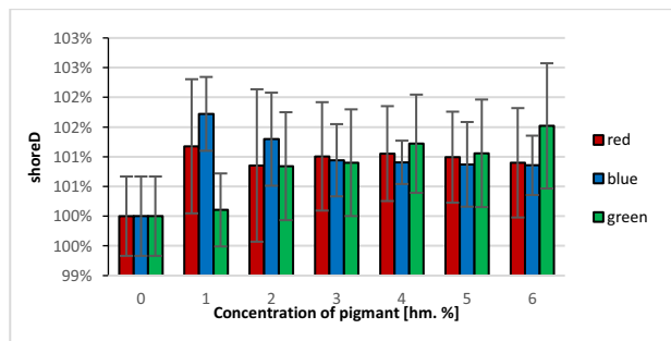
Fig 10. Proportional graph ShoreD
