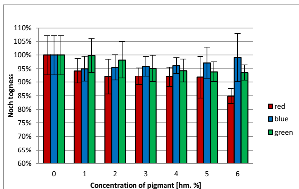
Fig 6. Proportional graph of notch toughness
