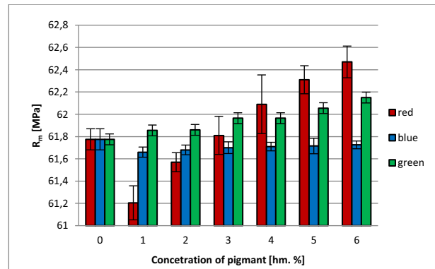
Fig 7. Limit of strength
