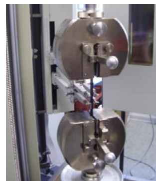
Fig 4. Tensile stress experiment
