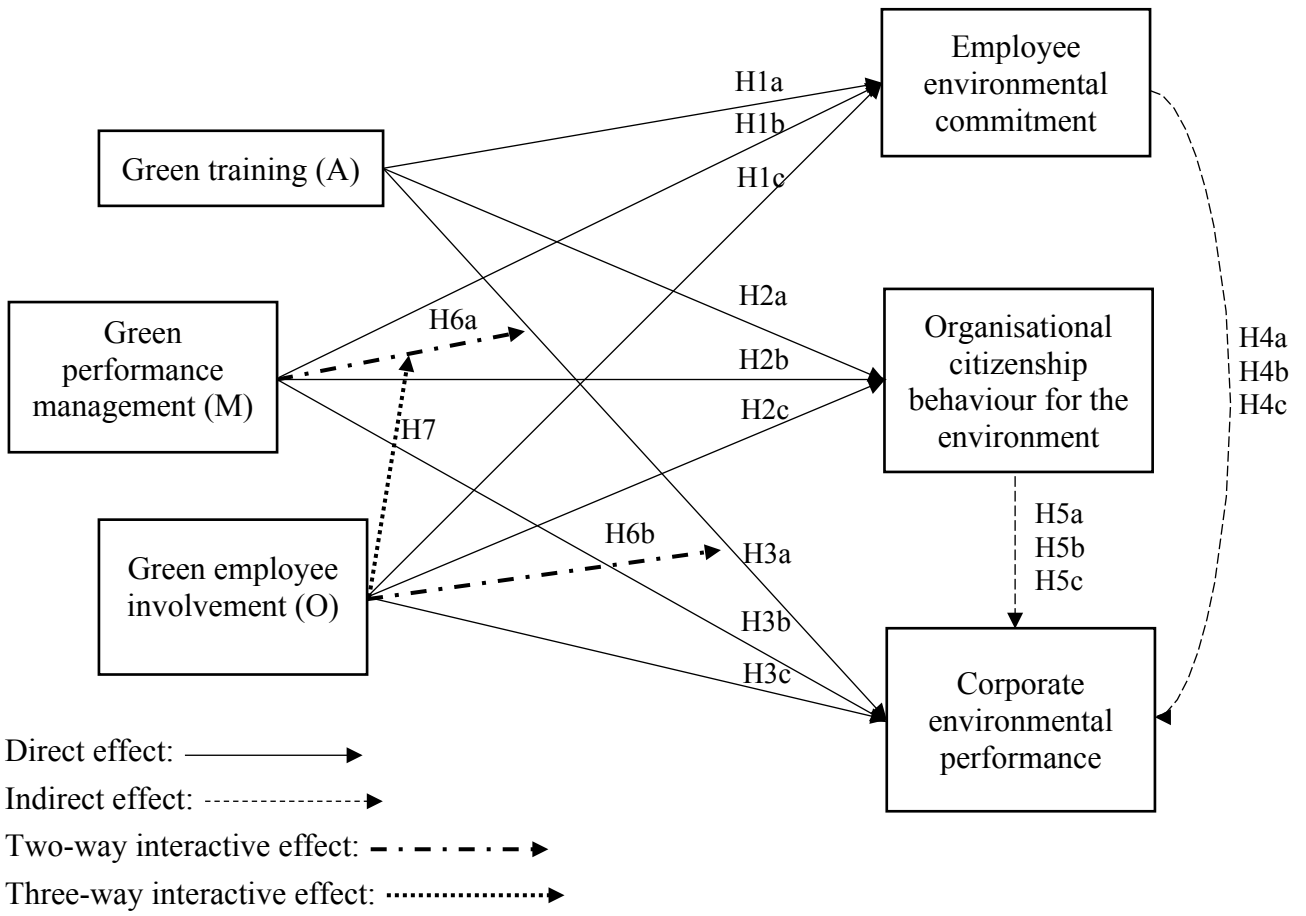
Fig. 1. Conceptual model.
