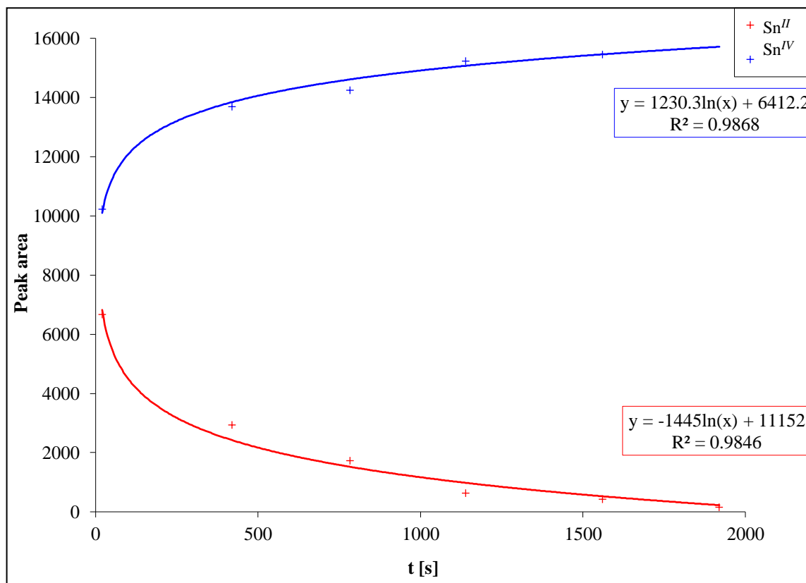
Figure 3 Logarithmical dependence of conversion of Sn (II) on Sn (IV).
