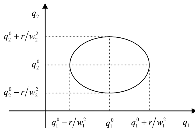
Figure 1. Ellipsoidal geometry defined by weighted Euclidean norm [5,15].
