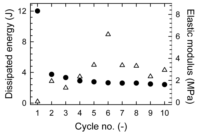
Figure 9: Results of the cyclic closed shell compression loading experiments of the calcium carbonate (sample 1) (deformation rate 10 mm/min, maximum force 80 kN): full circle – dissipated energy (J), triangle up – elastic modulus (MPa)
