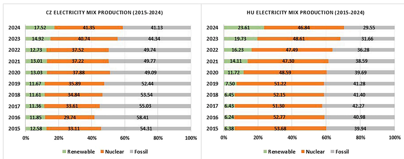
Figure 3. Electricity production, excluding import of electricity, in the Czech Republic and Hungary in 2015–2024 (energy-charts)
