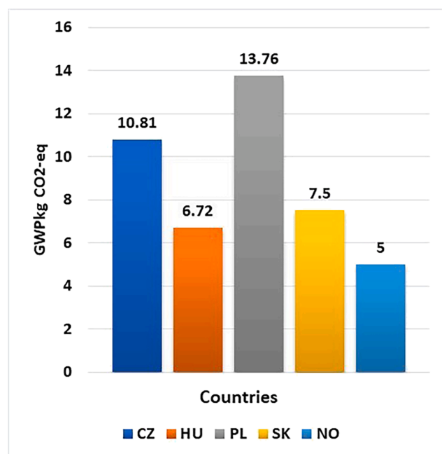
Figure 5. GWP of energy demand per kWh (electricity and heat) during battery production, 2024 electricity mix
