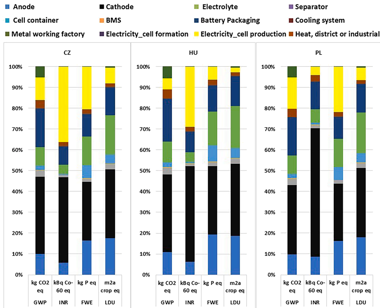
Figure 6. Impacts of 1 kWh of NMC 811 battery production on GWP, INR, FWE, and LDU in CZ, HU, and PL, 2024 electricity mix
