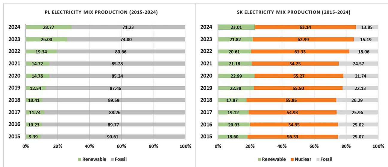
Figure 4. Electricity production, excluding import of electricity, in Poland and Slovakia in 2015–2024 (energy-charts)
