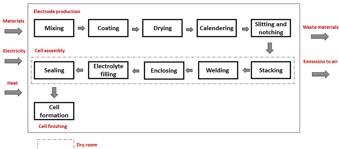
Figure 8. Process flow diagram of cell production
