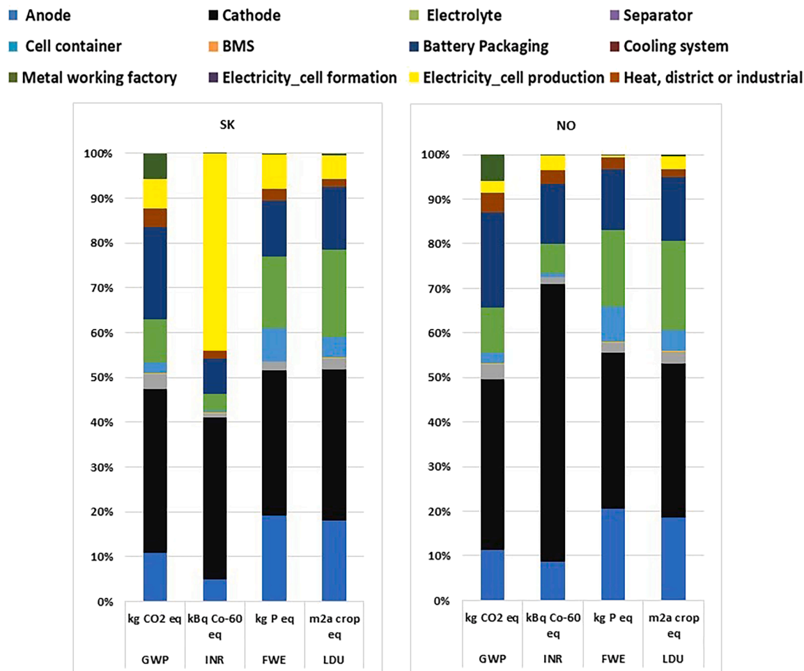
Figure 7. Impacts of 1 kWh of NMC 811 battery production on GWP, INR, FWE, and LDU in SK and NO, 2024 electricity mix
