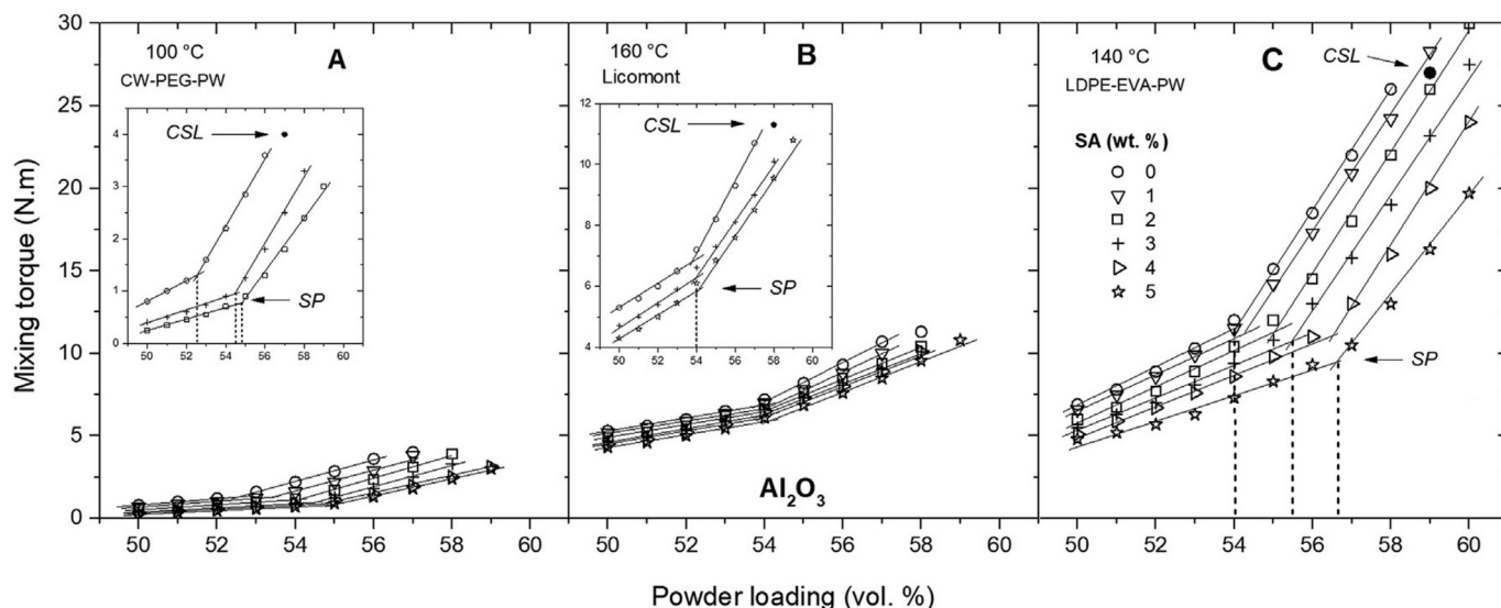
Fig. 2. Evaluation of critical solid loading (CSL) and switch point (SP) from torque dependence on \text{Al}_2\text{O}_3 powder loading in feedstocks differing in binder composition (with permission from [97]).
