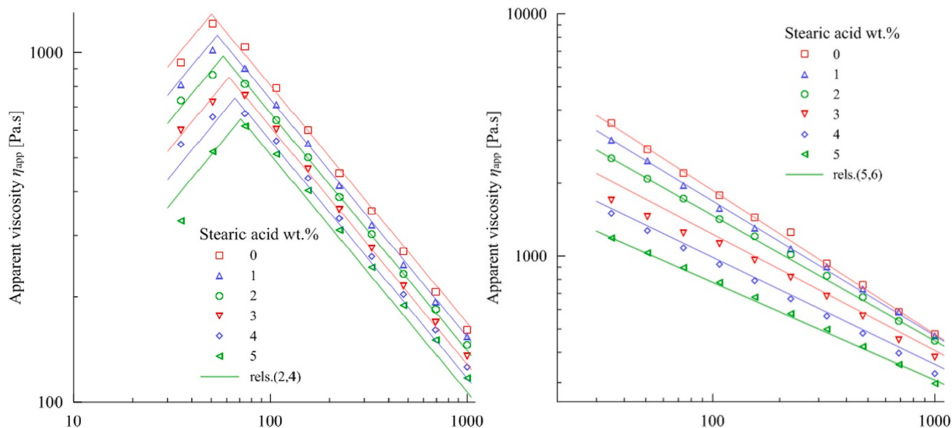
Fig. 5. Approximation of apparent viscosity of dilatant/pseudoplastic (Licomont commercial binder) and pseudoplastic (CW/PW/PEG binder) \text{Al}_2\text{O}_3 feedstocks with master curves (with the permission from [97]).
