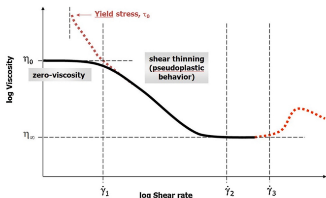
Fig. 4. Typical flow curve of highly filled compounds exhibiting yield stress and dilatancy (red-dotted) compared to typical flow curve of polymer melts (with the permission from [103]).
