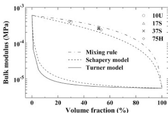
Fig. 7. Bulk moduli of various carbide compounds varying in particle size distribution as a function of powder volume fraction. The dash-dot line represents the prediction according to the mixing rule, the dashed and full lines represent the boundaries of Schapery and Turner models, respectively (with permission from [123]).
