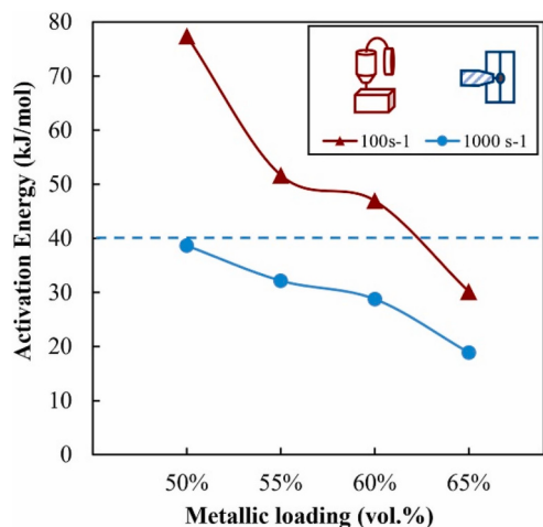
Fig. 6. Activation energy as a function of powder loading for typical MEX and PIM shear rates (with permission from [113]).
