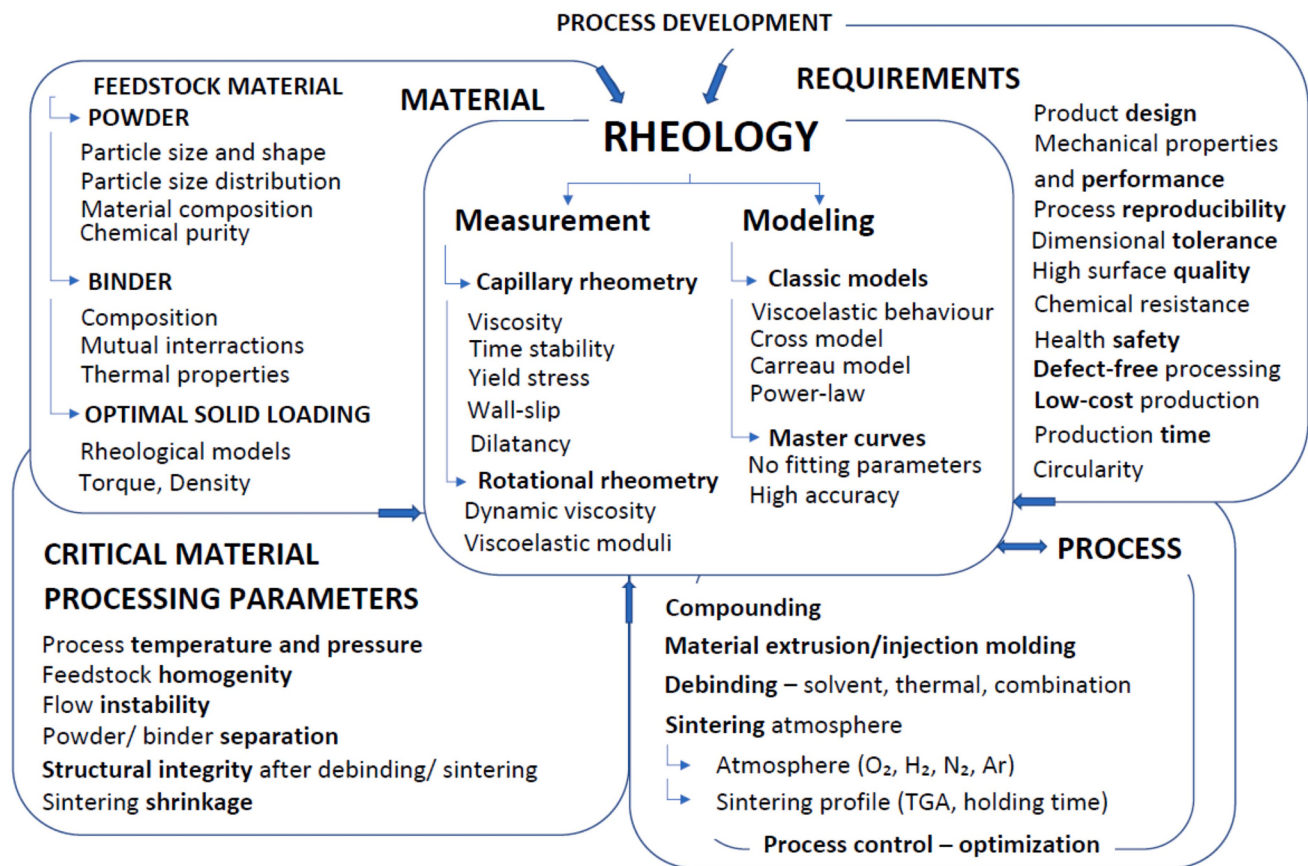
Fig. 1. Role of rheology in feedstock design and process development for MEX and PIM.
