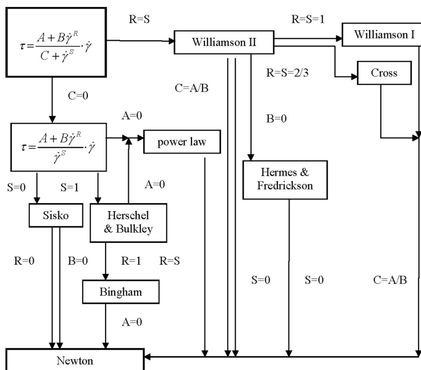
Fig. 3. Overview of relevant basic rheological models for MEX and PIM feedstocks (with the permission from [102]).
