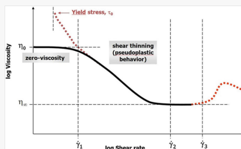
Typical flow curve of highly filled compounds exhibiting yield stress and dilatancy (red-dotted) compared to typical flow curve of polymer melts (with the permission from [103]).
