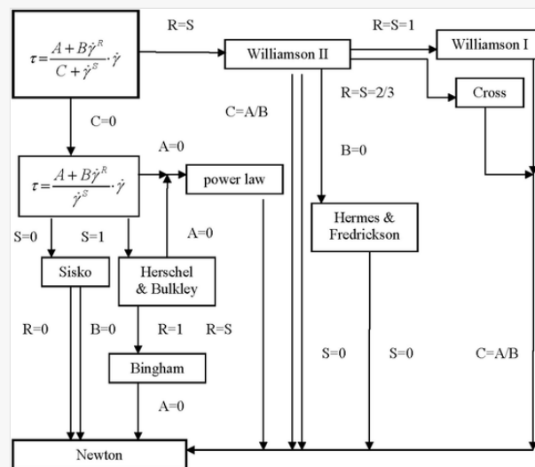
Overview of relevant basic rheological models for MEX and PIM feedstocks (with the permission from [102]).
