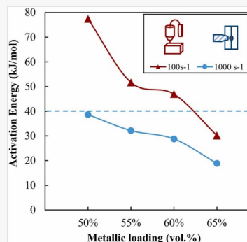
Activation energy as a function of powder loading for typical MEX and PIM shear rates (with permission from [113]).
